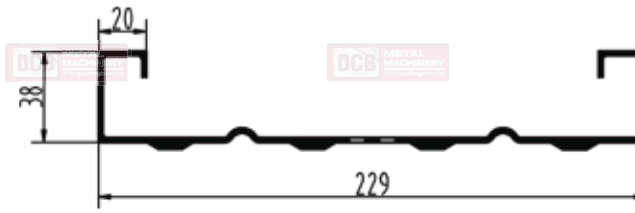
2. Kwikstage Steel Plank
