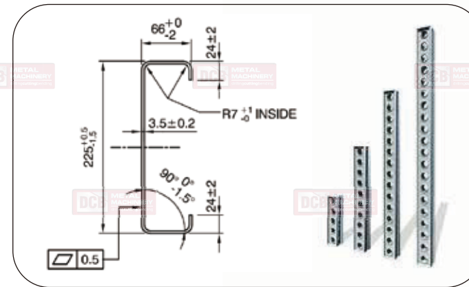
1. Superslim soldier channel
