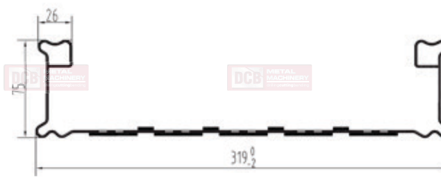
1. Ringlock Steel Deck O Type
