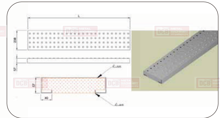
2. Omega cuplock board
