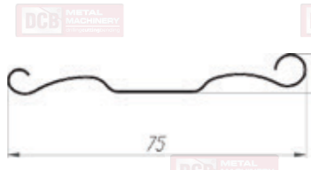
Profile Drawing
