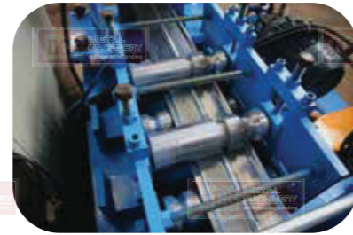
Forming Rollers
